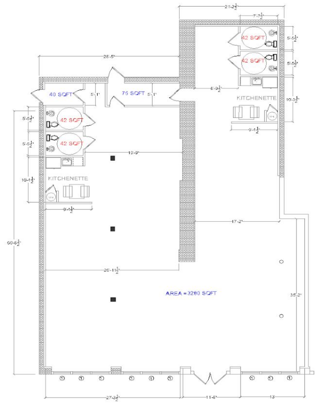
1617 EASTERN AVE - COMMERCIAL SPACE - OPEN SCALE: 3/16=1'-0"
