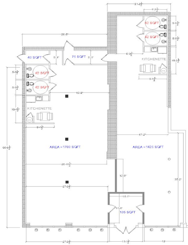
1617 EASTERN AVE - COMMERCIAL SPACE - SPLIT SCALE: 3/16=1'-0"
